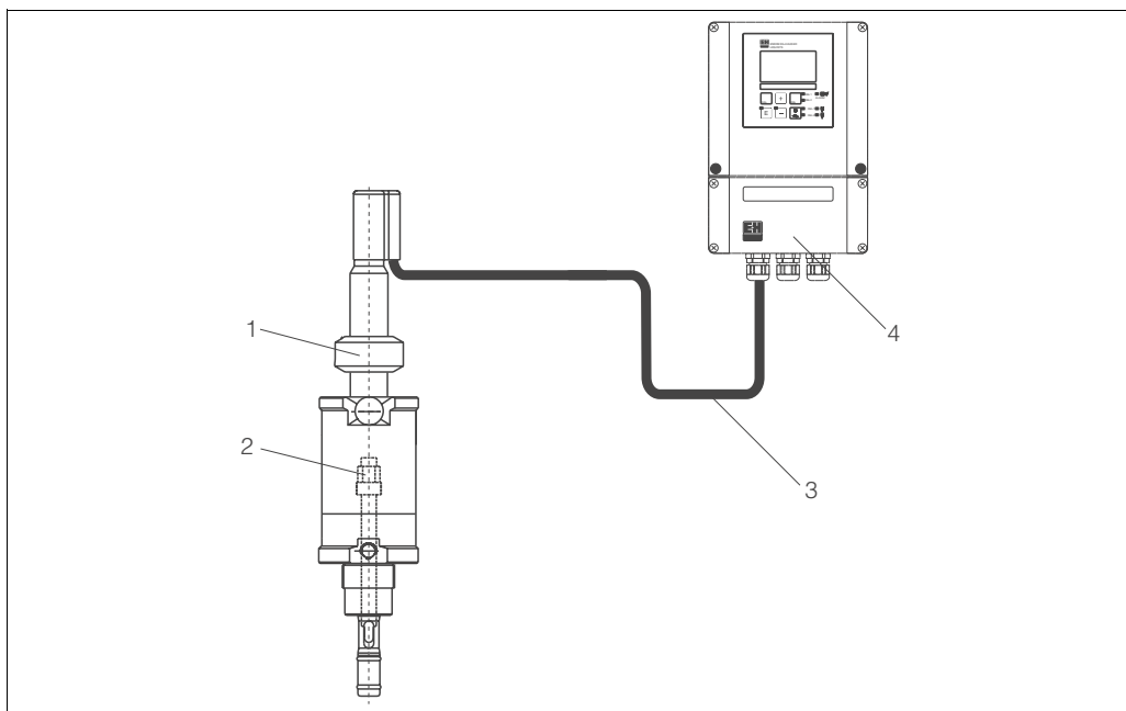
Measuring system for pH measurement
